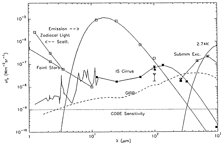
Figure 1. The IR background due to galaxies (GIRB, dashed line) among the various foregrounds and backgrounds (see text).
