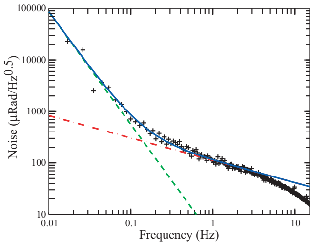
Fig. 10. LEKID phase-noise spectrum measured during a total power scan (+, black) under normal daytime conditions ( \tau \sim .2 at 225 GHz). The roll-off above 5 Hz is related to the readout electronics rate. The solid line (blue) is a fit of N_{\theta} = Af^{\alpha} + Bf^{\beta} to the data below 5 Hz ( \alpha = -0.43 , \beta = -2.19 ). The dashed line (green) is a plot of the fitted Af^{\alpha} term which is predominately caused by sky fluctuations. The dash-dot line (red) is a plot of the Bf^{\beta} term which is dominated by intrinsic detector noise. No change in the intrinsic detector noise or spurious electrical noise was observed upon moving from the laboratory to the telescope environment.
