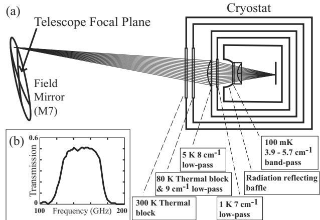
Fig. 3. NIKA optical configuration. a) The IRAM telescope focal plane coincides with the M7 tangential plane. M7 is a bi-polynomial mirror interfacing the NIKA instrument with the telescope optics. b) Calculated transmission of the filter stack, based on measurements of the individual elements. The bandpass is from 125 to 170 GHz.
