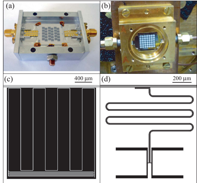
Fig. 2. Array and single-pixel images. a) LEKID 30 pixel array and b) antenna-coupled 42 pixel array with sapphire microlenses. The dimensions of the focal plane are in both cases \sim 1 \text{ cm}^2 , corresponding to a 45 arcsec field-of-view. c) Single LEKID resonator design and d) antenna-coupled resonator design. For both designs, a high quality metallic film is first deposited onto a dielectric wafer. A subsequent etching process is then used to remove metal in the black regions.
