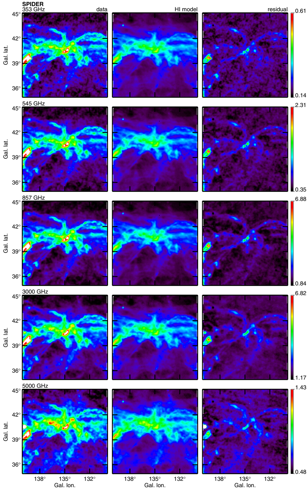
Fig. 9. Like Fig. 4, for field SPIDER.
